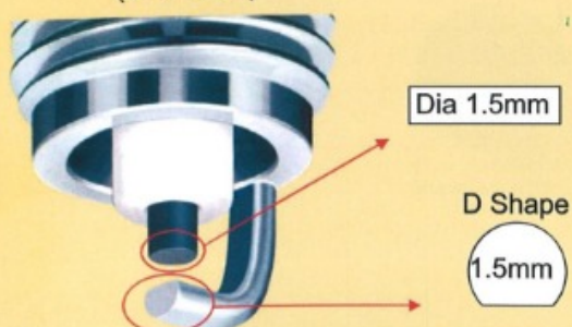
*31917-KWP-D01 (MR7C-9N)
