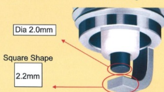
Normal Plug
